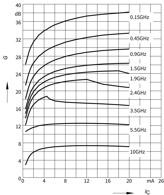
Figure 8 Maximum power gain G_{max} = f(I_C) , V_{CE} = 3\text{ V} , f = \text{parameter in GHz}
