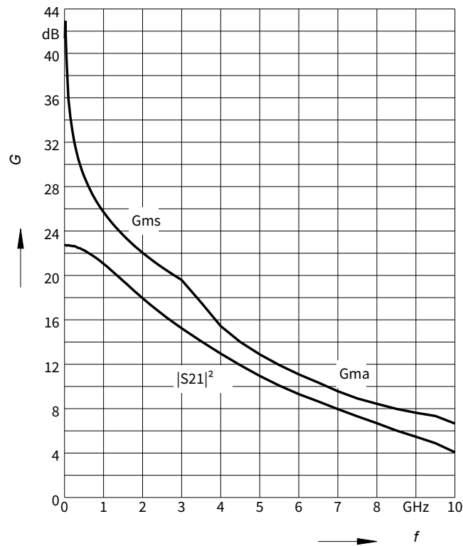
Figure 7 Gain G_{ma} , G_{ms} , |S_{21}|^2 = f(f) , V_{CE} = 3\text{ V} , I_C = 5\text{ mA}
