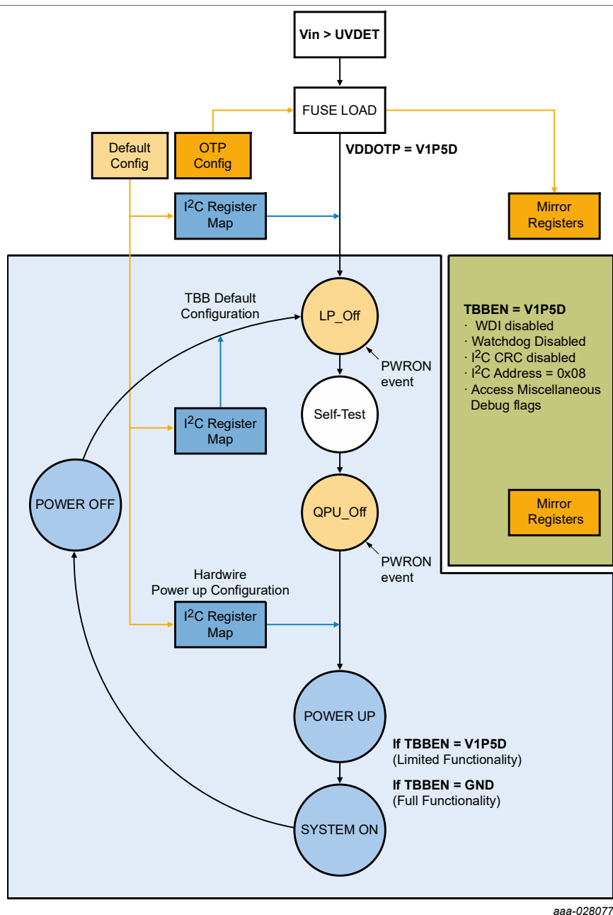
Figure 40. Hardwire operation diagram
