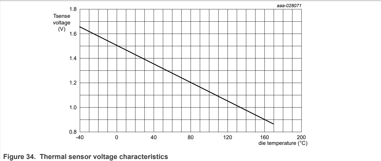
Figure 34. Thermal sensor voltage characteristics
