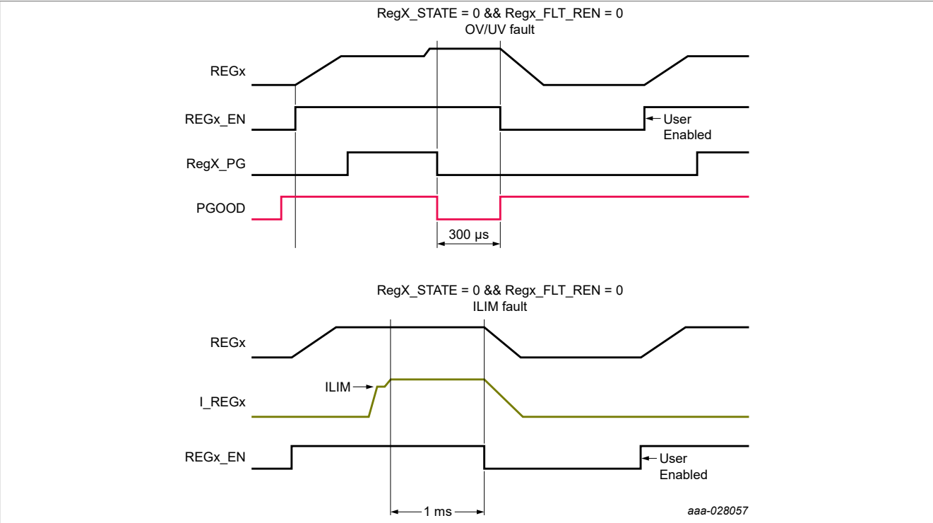
Figure 12. Regulator turned off with RegX\_STATE = 0 and FLT\_REN = 0
