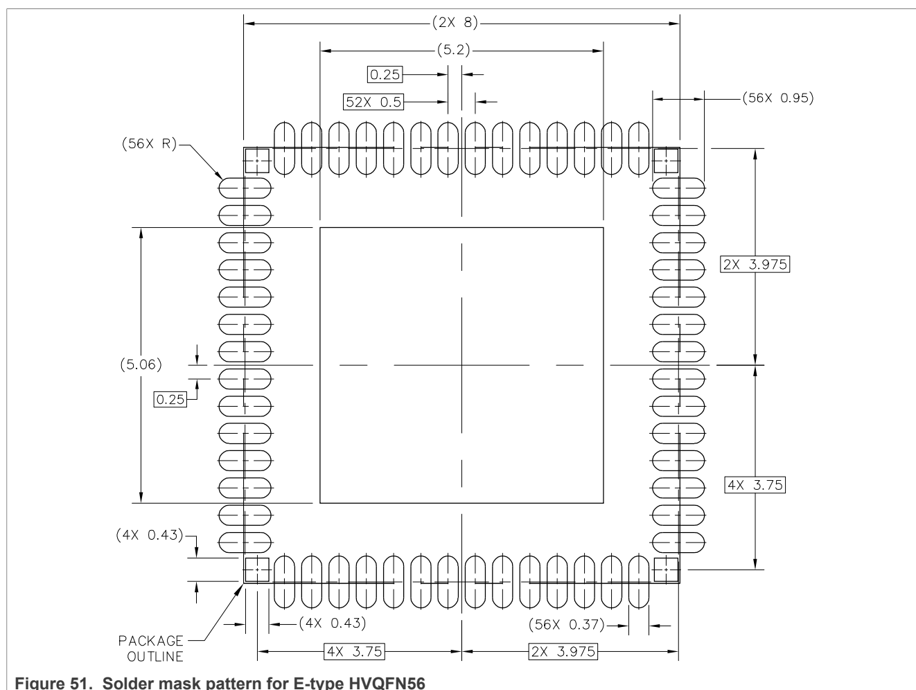
Figure 51. Solder mask pattern for E-type HVQFN56
