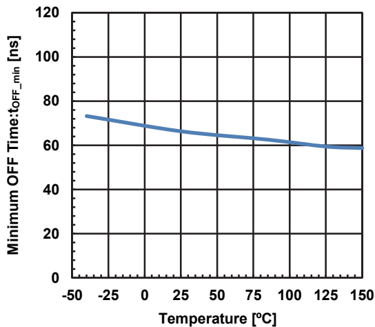
Minimum OFF Time vs. Temperature ( V^*=12\text{V} , R_T=7.32\text{k}\Omega )
