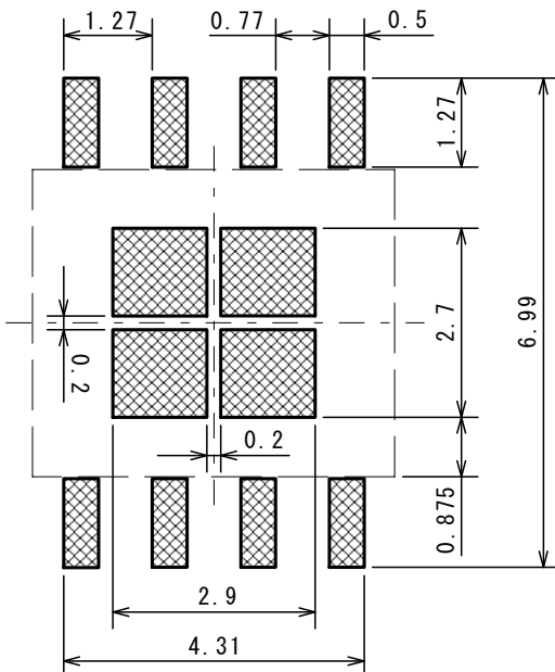
<Metal mask>
