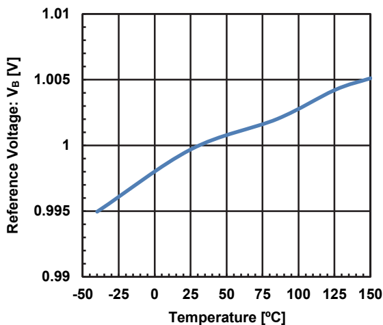
Reference Voltage vs. Temperature ( V^*=12\text{V} )
