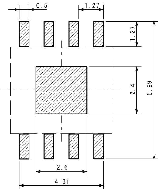
<Solder pattern>
