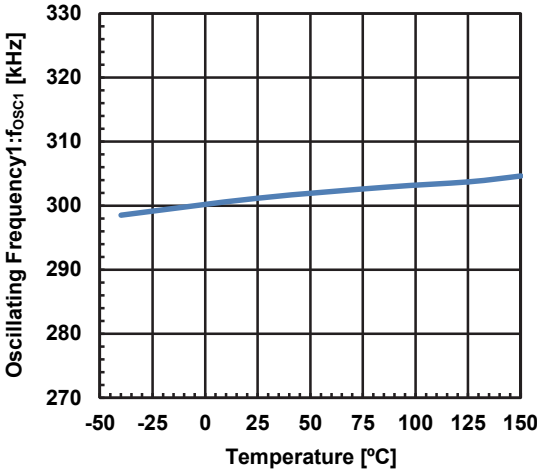
Oscillating Frequency vs. Temperature ( V^*=12\text{V} , R_T=27\text{k}\Omega )
