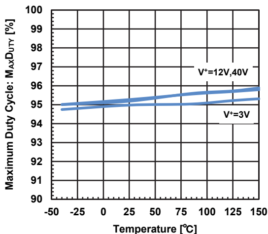
Maximum Duty Cycle vs. Temperature ( R_T=27\text{k}\Omega )
