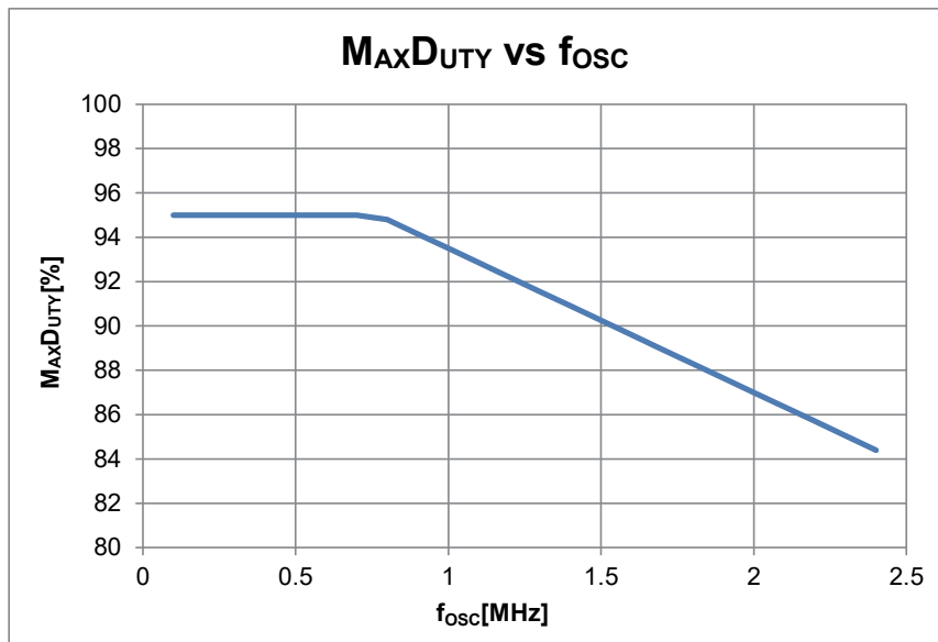
Fig.1 Maximum duty cycle vs. oscillation frequency.
