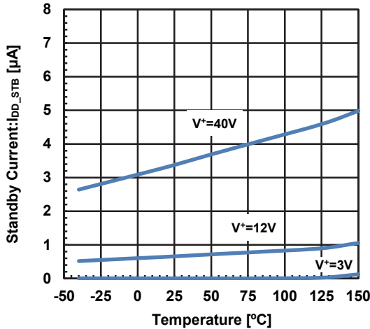
Standby Current vs. Temperature ( V_{EN}/\text{SYNC}=0\text{V} )
