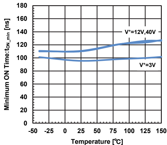
Minimum ON Time vs. Temperature ( R_T=27\text{k}\Omega )
