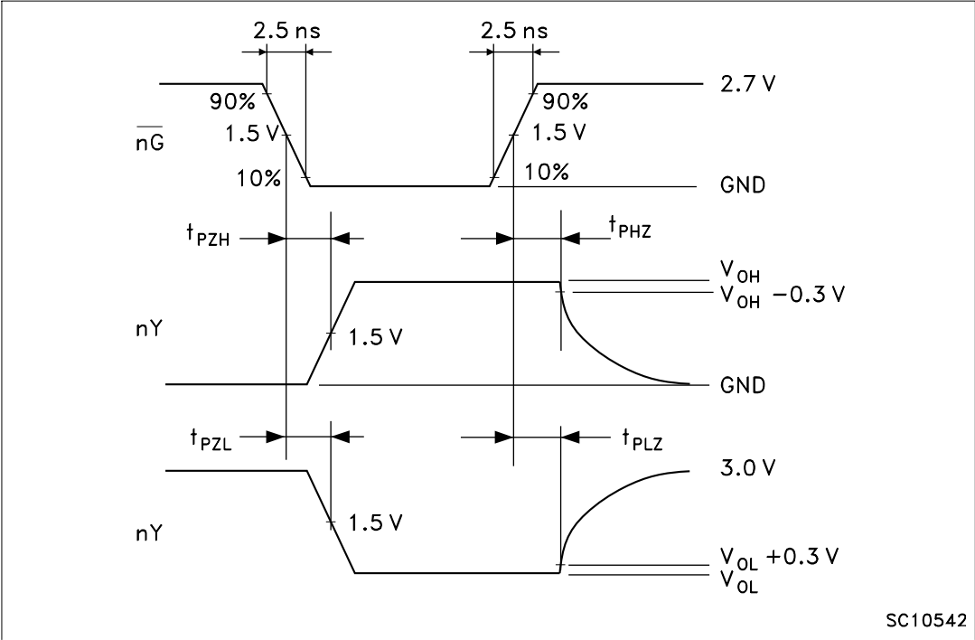
Figure 6. Output enable and disable time ( f = 1\text{ MHz} ; 50% duty cycle)
