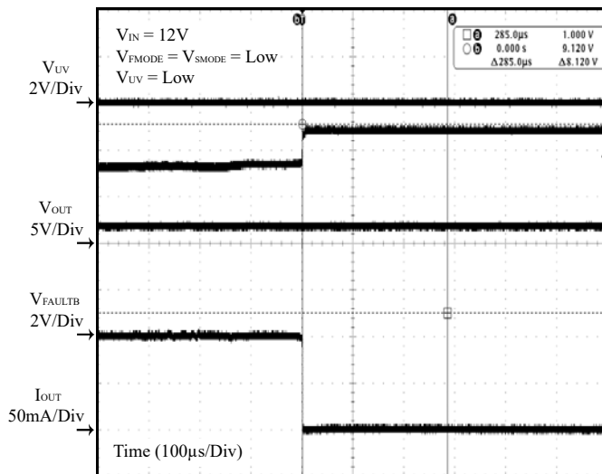
Figure 29 Output Open
