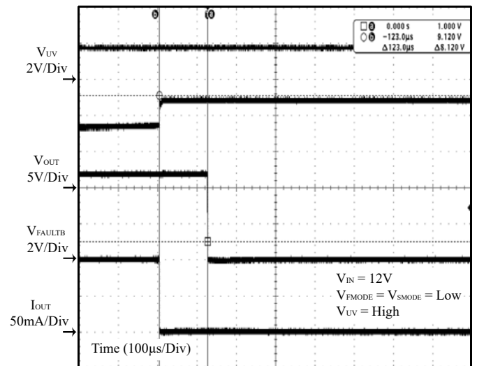
Figure 30 Output Open
