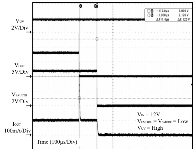
Figure 34 Output Short
