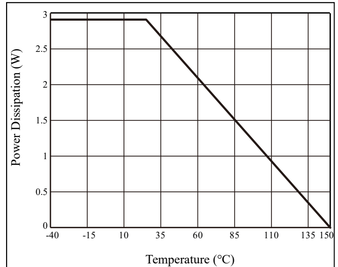
Figure 54 Dissipation Curve
