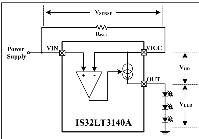
Figure 47 Voltage Drop
