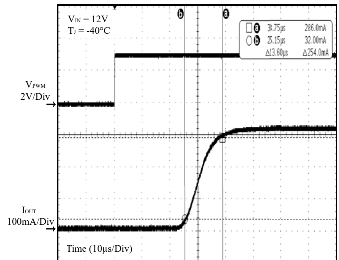
Figure 22 PWM On
