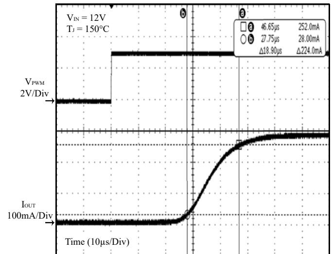
Figure 28 PWM On
