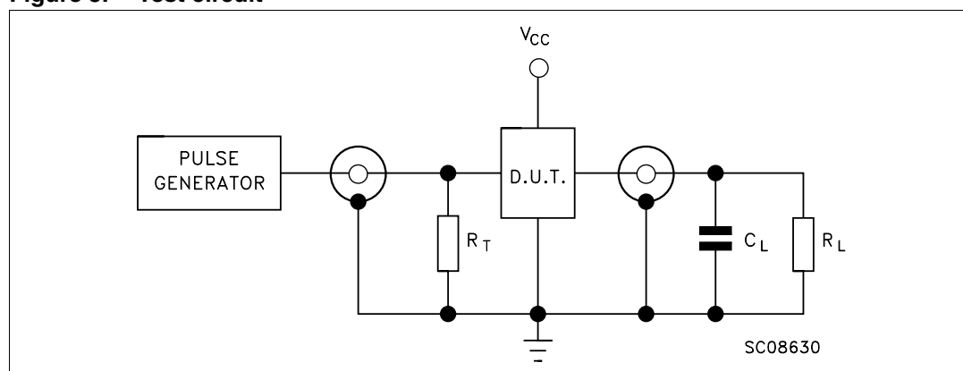
Figure 5. Test circuit
