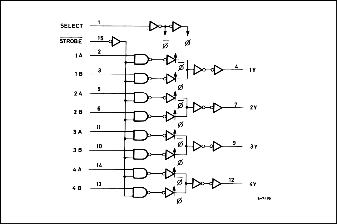
Figure 4. Logic diagram
