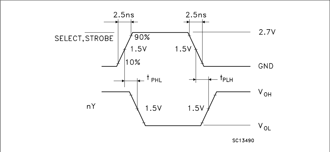
Figure 6. Propagation delay for inverting outputs (f = 1MHz; 50% duty cycle)
