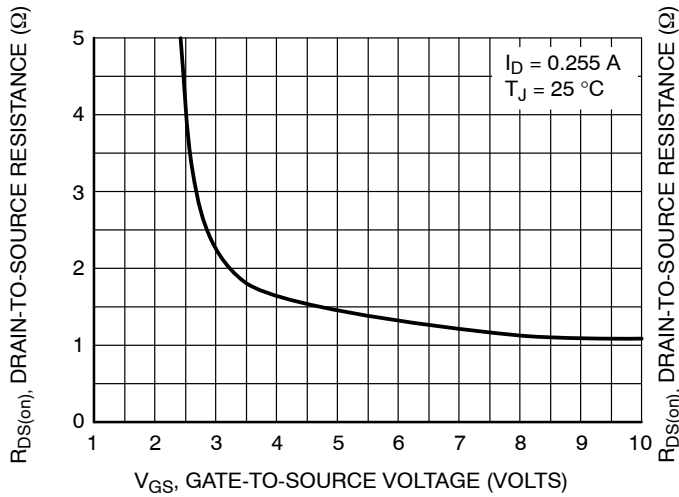
Figure 3. On-Resistance vs. Gate-to-Source Voltage
