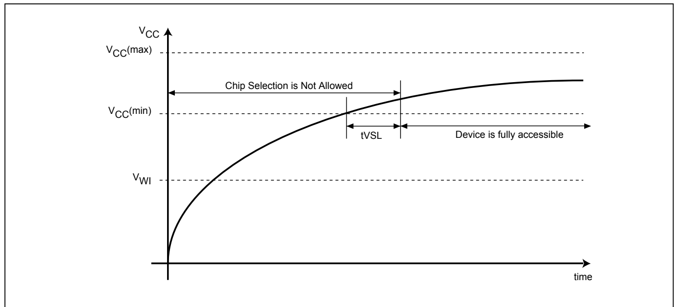
Figure 47. Power-up Timing
