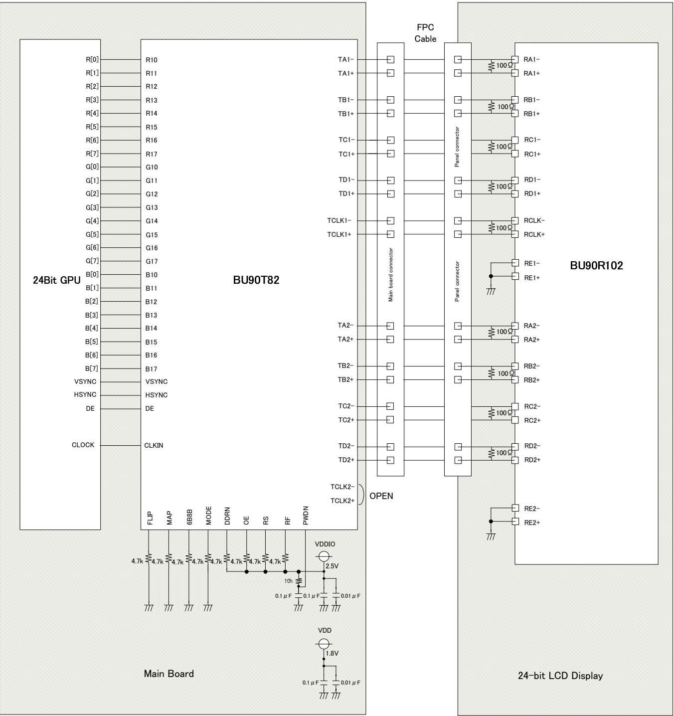
Figure 21. Application Circuit (24bit Dual-out mode)
