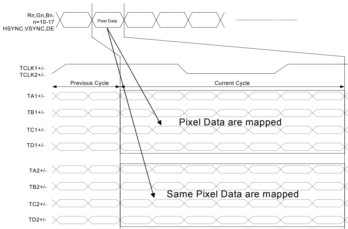
Figure 13. Single-In/Distribution-out Mode (FLIP=L)
