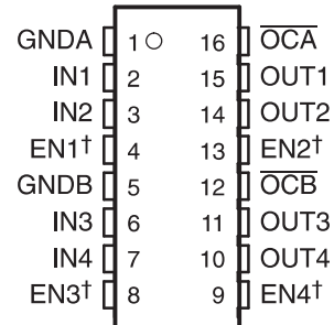
TPS2095, TPS2096 AND TPS2097
