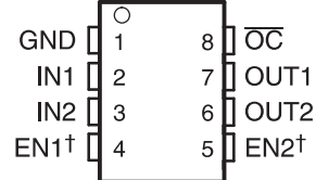
TPS2090, TPS2091, AND TPS2092
