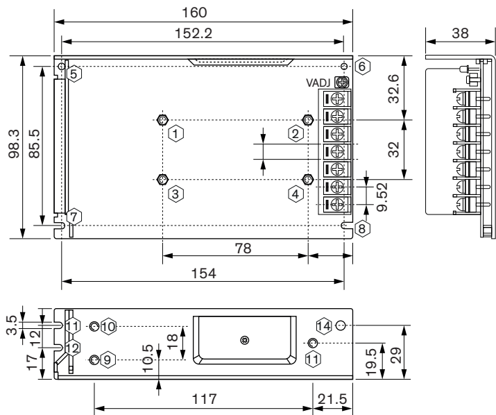
Dimensions in mm (inch) Outside dimension tolerance: ±1.0 (±0.04)
