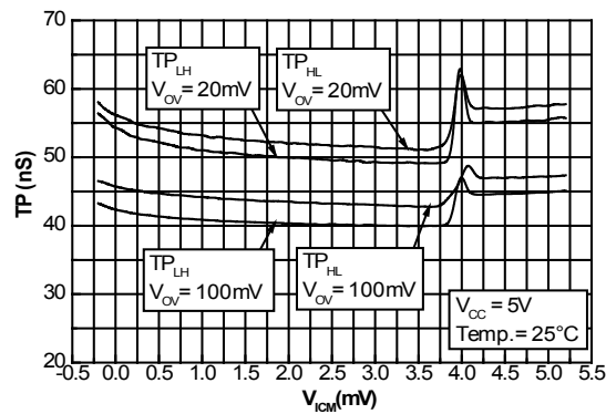
Figure 28. Propagation delay vs. common mode voltage, V_{CC} = 5\text{ V}
