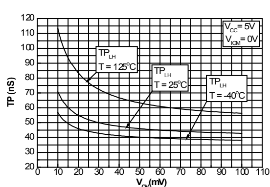
Figure 25. Propagation delay (LH) vs. overdrive at V_{CC} = 5\text{ V} , V_{ICM} = 0\text{ V}
