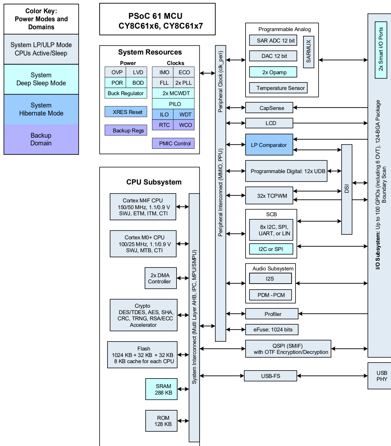
Figure 3. Block Diagram
