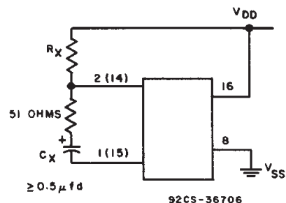
Fig. 18 - Alternate rapid power-down protection circuit.
