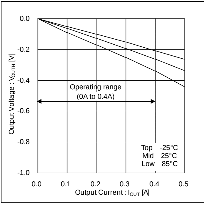
Figure 4. High Side Output Voltage vs Output Current
