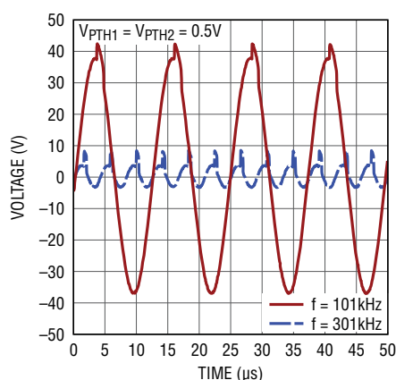
Figure 11. Comparison of the LC Tank Voltage Frequency without and with the Presence of a Conductive Foreign Object
