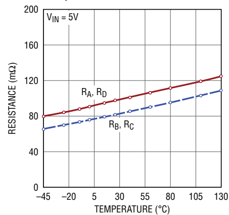
Switch Resistances Over Temperature
