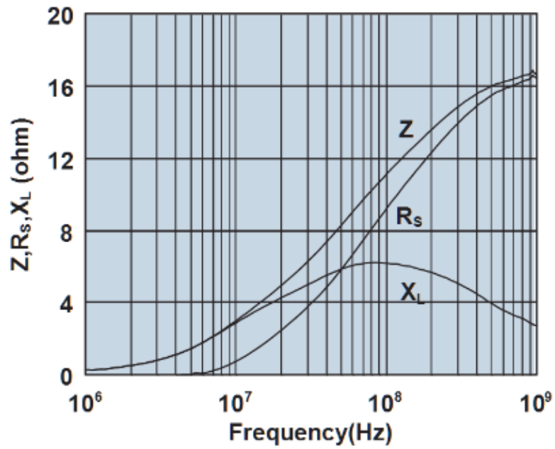
Impedance, reactance, and resistance vs. frequency.
