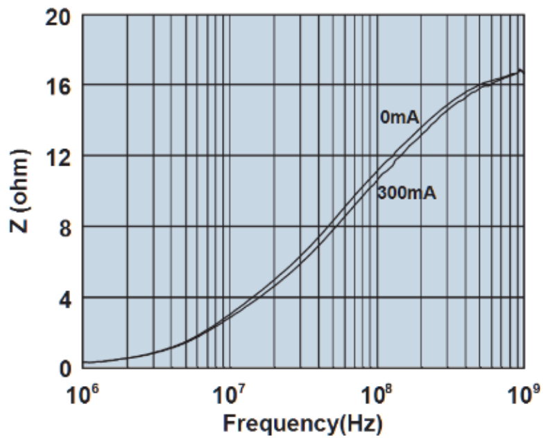
Impedance vs. frequency with dc bias.
