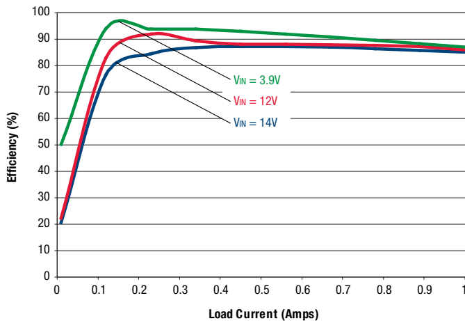
Efficiency vs. Line Voltage and Load Current @Ta = +25 °C (Vout = 3.3V)
