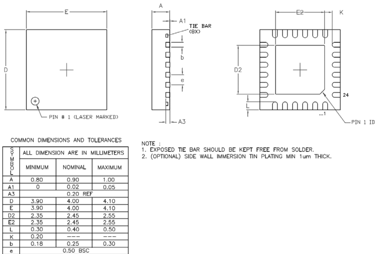
Figure 11: Package outline drawing and dimensions
