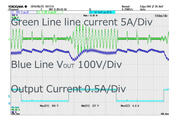
Figure 23. Load Transient V_{IN} = 90\text{ V}_{AC}
