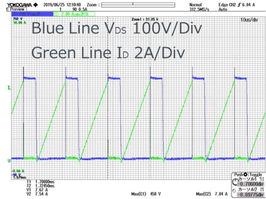
Figure 19. V_{DS}, I_D ZOOM
