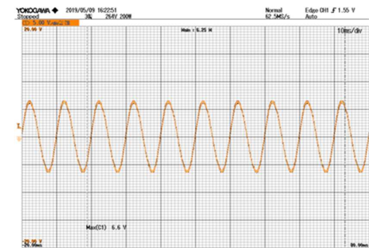
Figure 26. Output ripple V_{IN} = 264\text{ V}_{AC}
