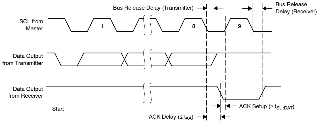
Figure 4. Acknowledge Timing
