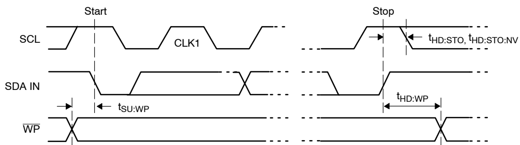
Figure 5. WP Timing
