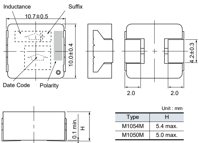
PCC-M1054M type PCC-M1050M type (ETQP5M□□□YFC/YGC)
