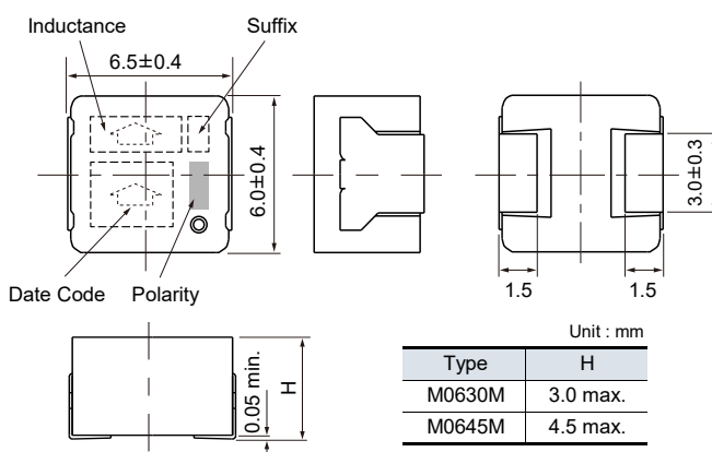
PCC-M0630M type PCC-M0645M type (ETQP3M□□□YFN/ETQP4M□□□YFN)
