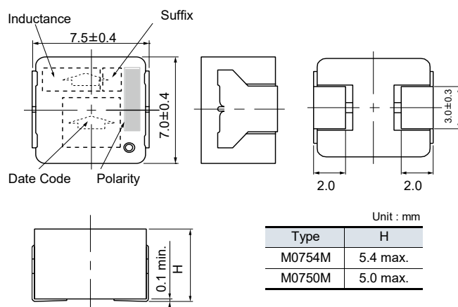
PCC-M0754M type PCC-M0750M type (ETQP5M□□□YFM/YGM)
