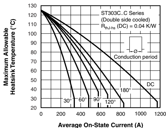
Fig. 4 - Current Ratings Characteristics
