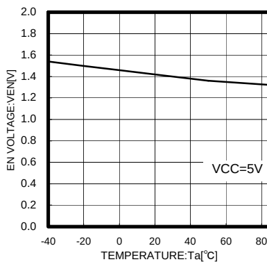
Fig.12 Ta – EN1, EN2
