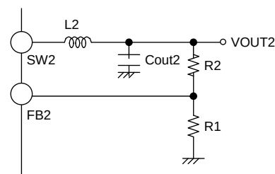
Fig.39 Determination of output voltage
