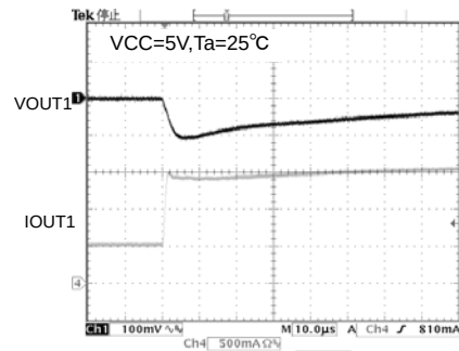
Fig.20 VOUT1 transient response ( I_o0.5A \rightarrow 1.5A / usec)
