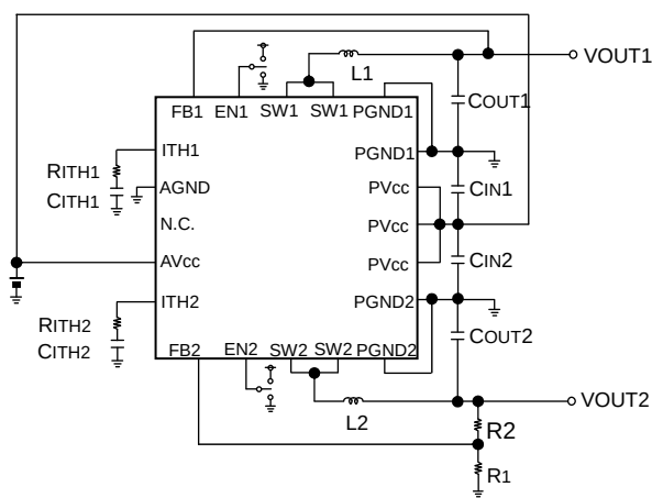
Fig.40 Layout diagram
