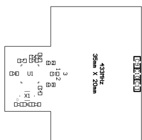
a) Top silk screen
