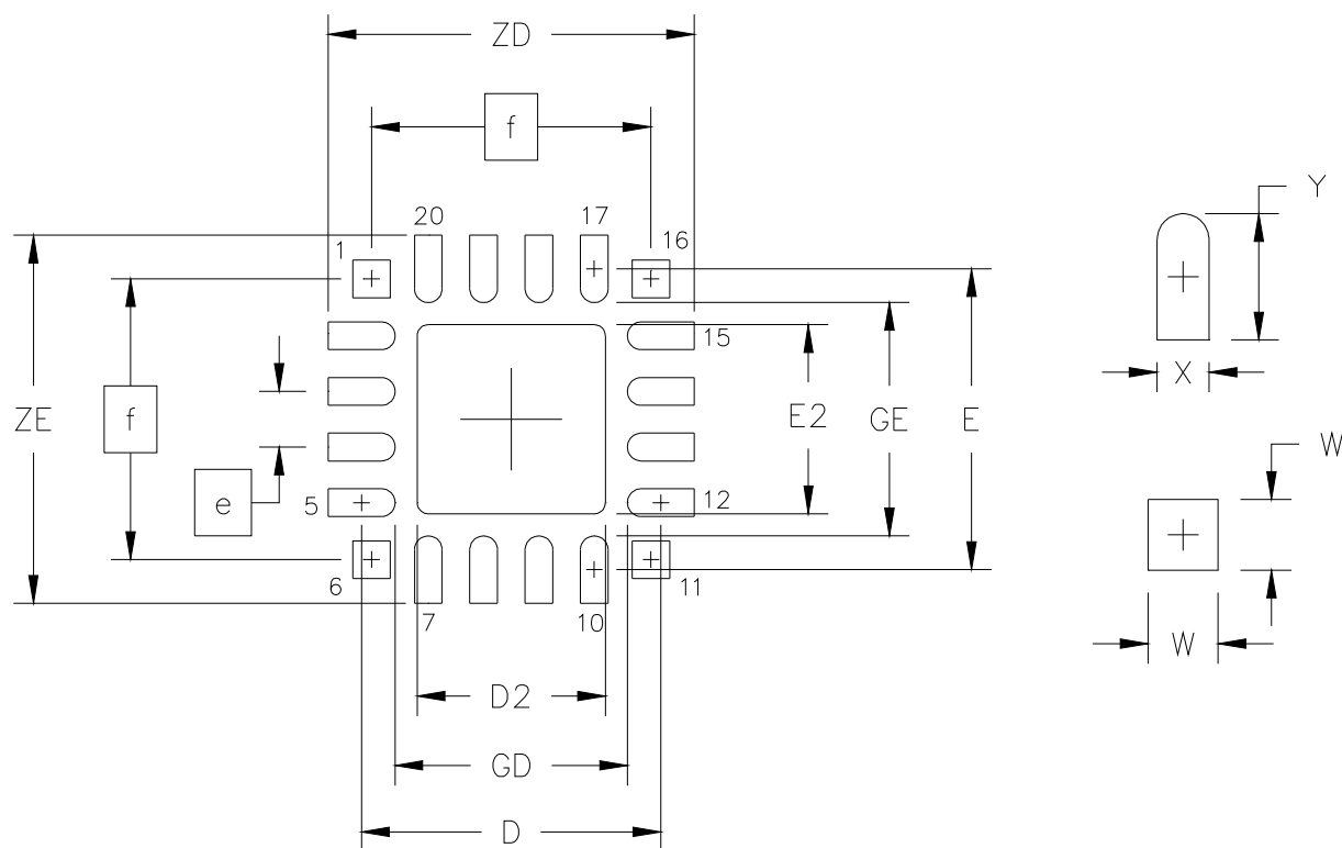
Figure 6. PCB Land Pattern
