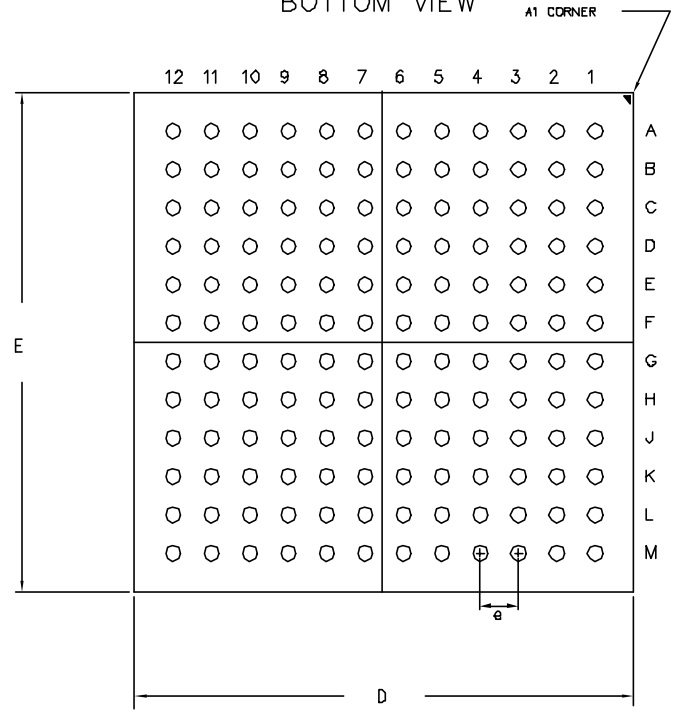
BOTTOM VIEW
