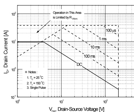
Figure 9-2. Maximum Safe Operating Area for FQPF10N20C
