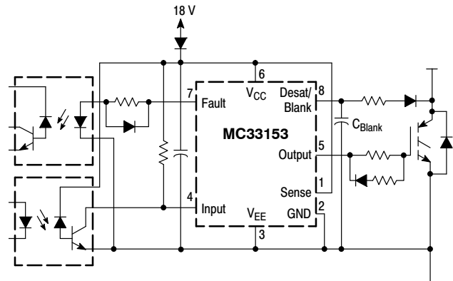
Figure 37. Desaturation Application
