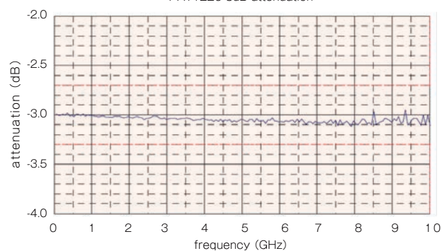
PAT1220 3dB attenuation
