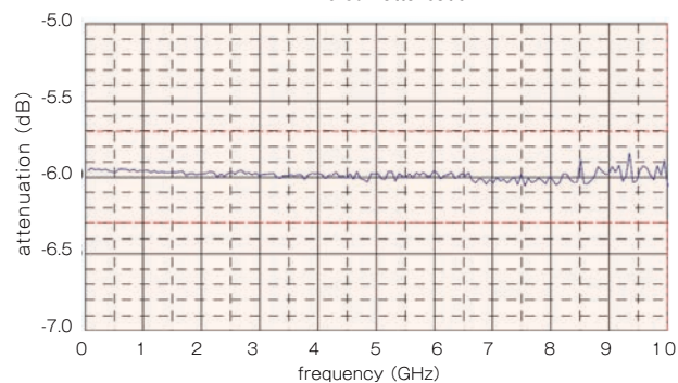
PAT1220 6dB attenuation
