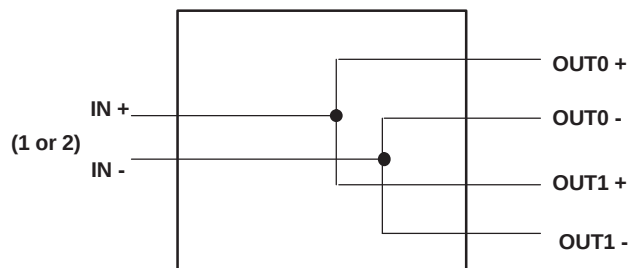
Figure 26. 1:2 Splitter
