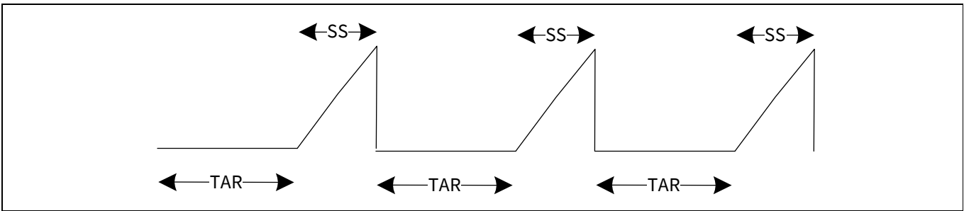
Figure 5 Auto-restart
