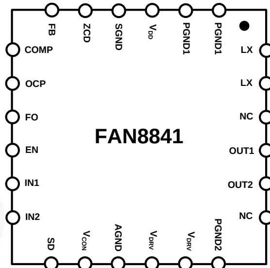
Figure 3. Pin Assignment
