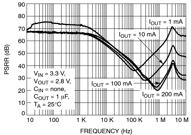
Figure 6. PSRR, V_{OUT} = 2.8 \text{ V} , C_{OUT} = 1 \mu\text{F}
