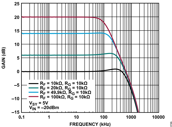
Figure 41. Inverting Small Signal Frequency Response
