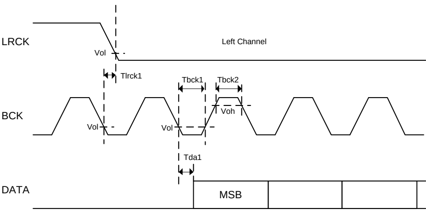
Figure 19 Timing chart
