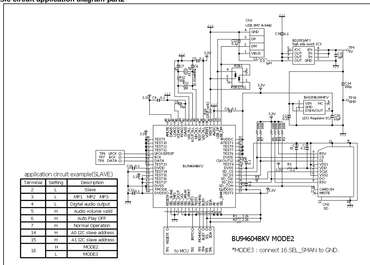
●Basic circuit application diagram-part2
