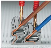
Testing with 2 mm Ø test plug – touch contact.
