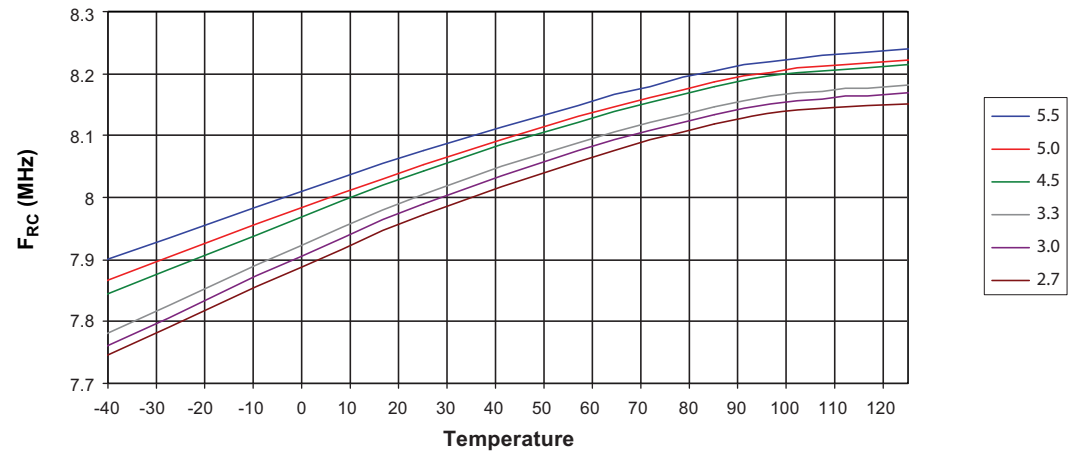
Figure 27-25. Calibrated 8MHz RC Oscillator Frequency versus Temperature
