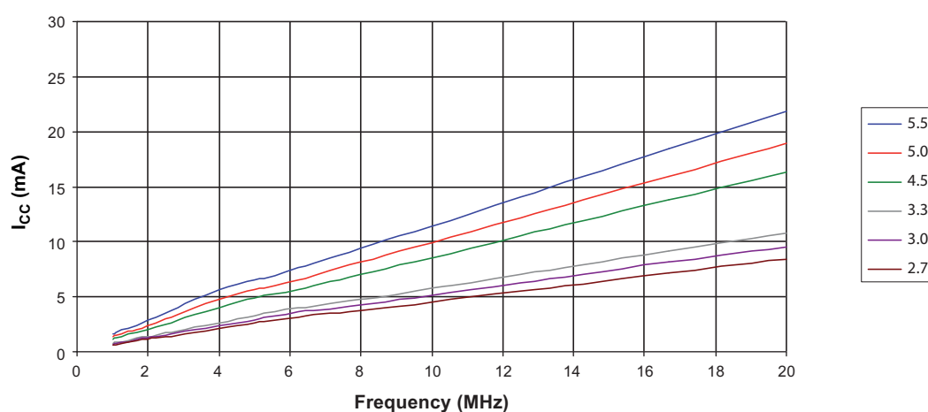
Figure 27-2. Active Supply Current versus Frequency (1 - 20MHz)
