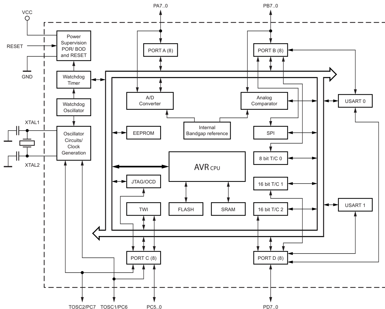
Figure 2-1. Block Diagram
