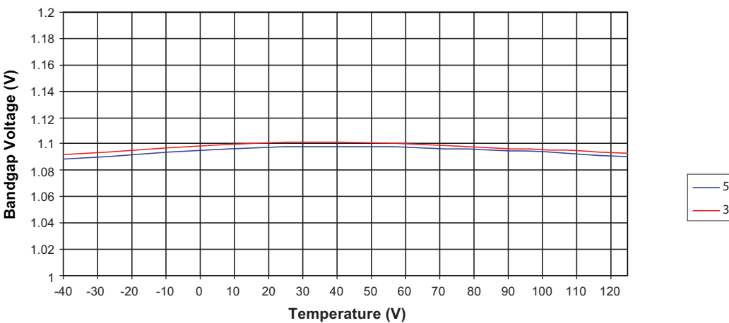
Figure 27-23. Bandgap Voltage versus Temperature
