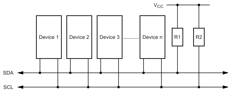
Figure 19-1. TWI Bus Interconnection
