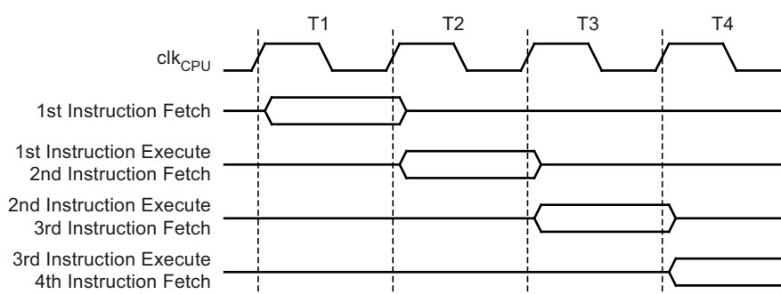
Figure 5-4. The Parallel Instruction Fetches and Instruction Executions
