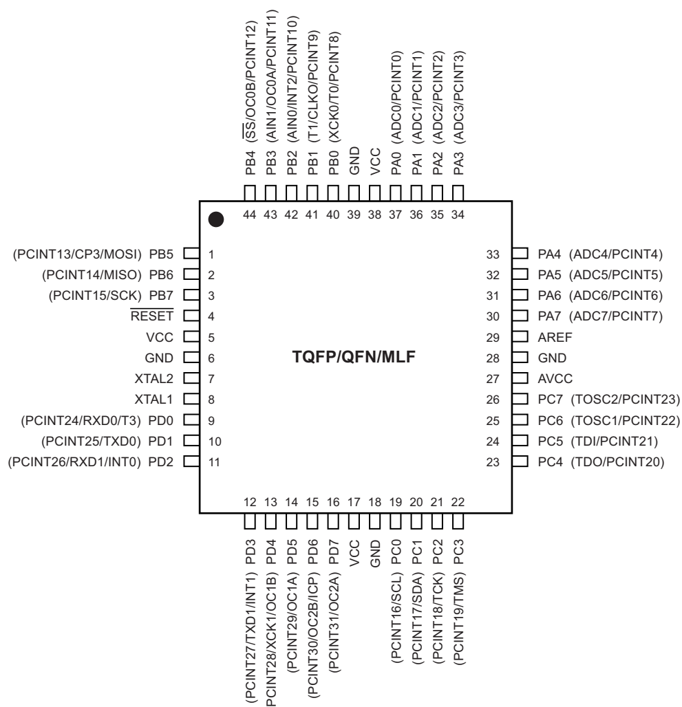
Figure 1-1. Pinout ATmega164P/324P/644P
