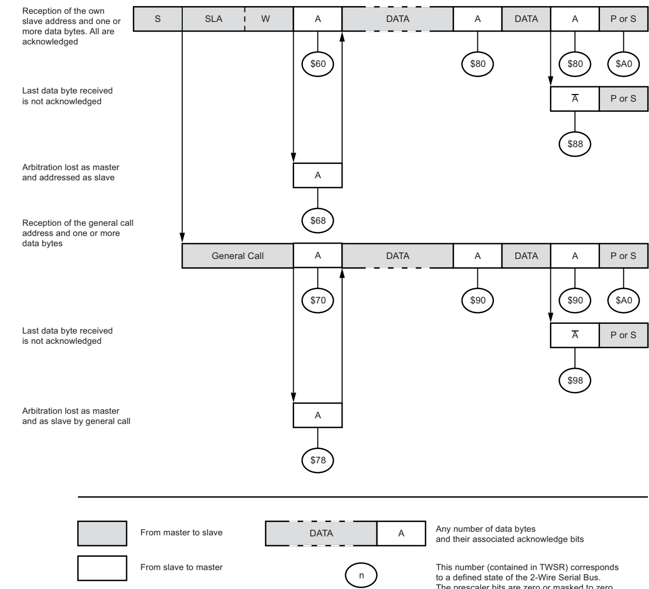
Figure 19-16. Formats and States in the Slave Receiver Mode
