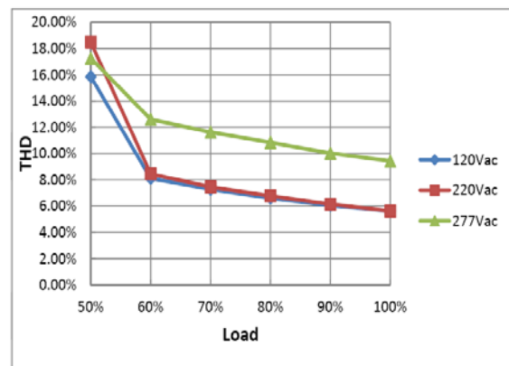
THD Curve
