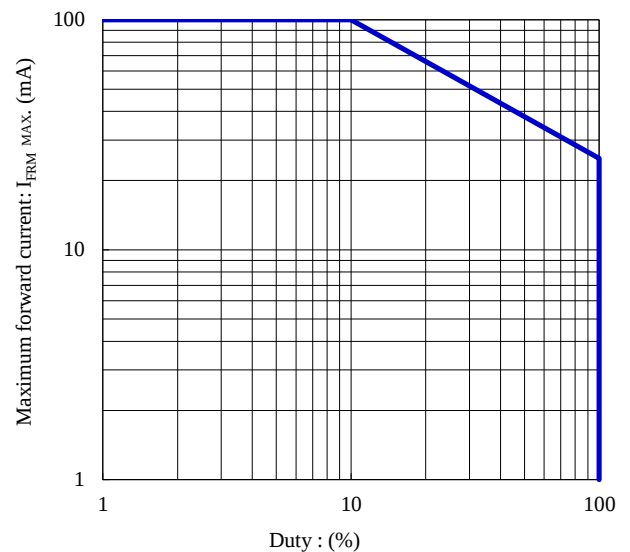
Duty cycle vs. Maximum forward current
