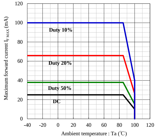
Ambient temperature vs. Maximum forward current
