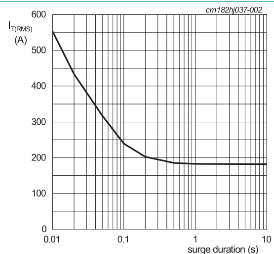
Fig. 2. RMS on-state current as a function of surge duration; maximum values f = 50\text{ Hz} ; T_{mb} = 107\text{ °C}
