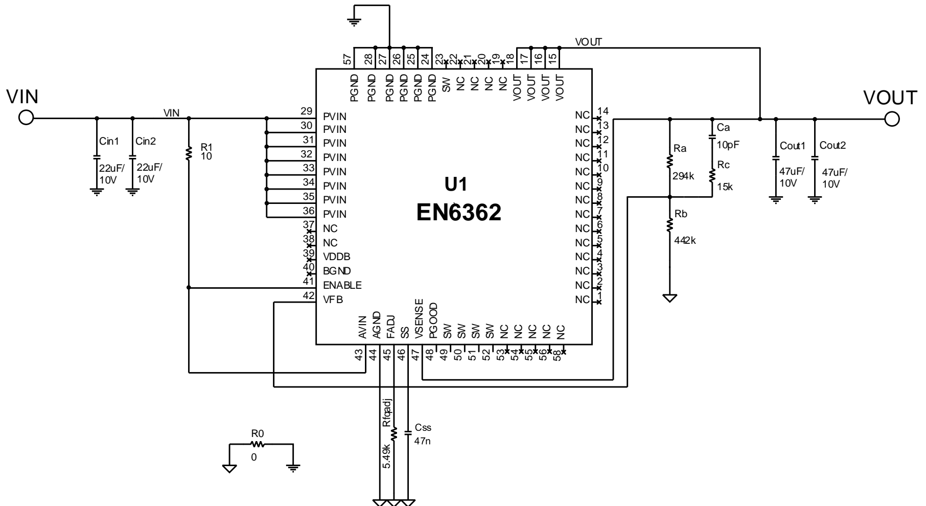
Figure 7: Application Schematic
