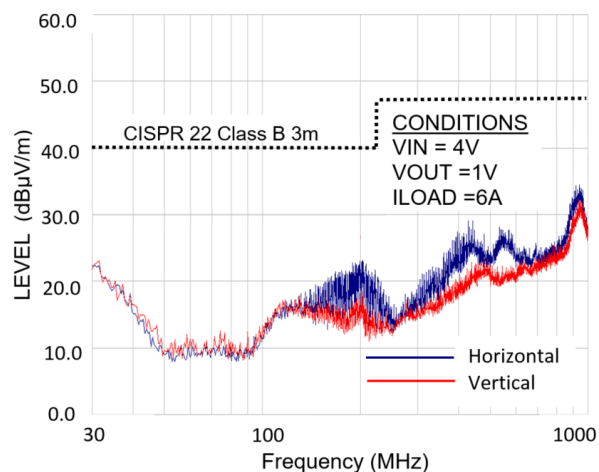
EMI Performance
