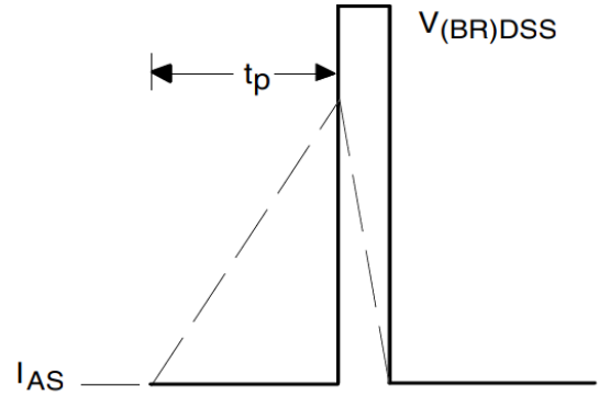
Fig 16b. Unclamped Inductive Waveforms
