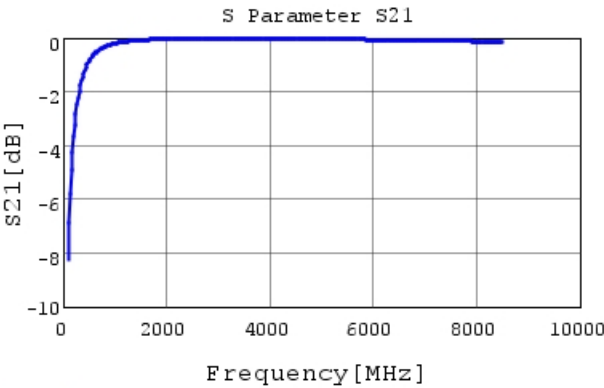
GCQ1555C1H6R7WB01 S21 DCOV, 25degC
