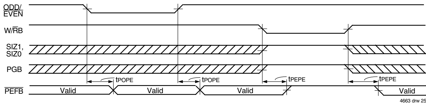
Figure 25. \overline{\text{ODD/EVEN}} , \overline{\text{W/RB}} , \text{SIZ1} , \text{SIZ0} , and \text{PGB} to \overline{\text{PEFB}} Timing
