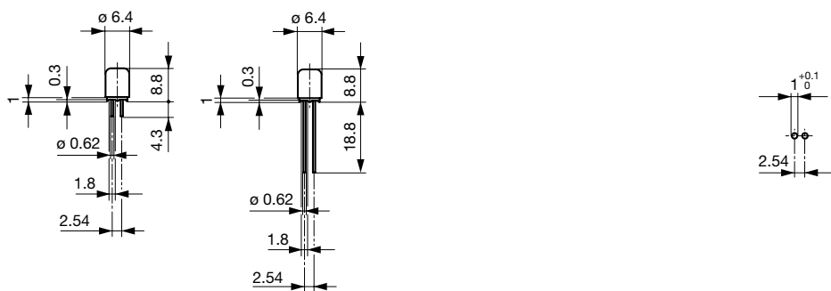
Drilling diagram
