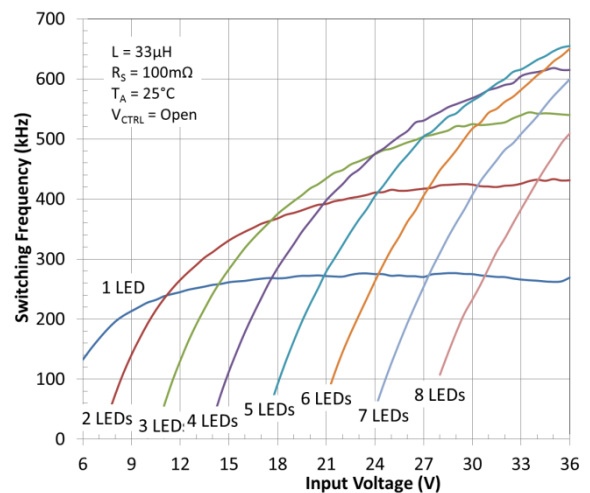
Figure 24. Switching Frequency vs. Input Voltage
