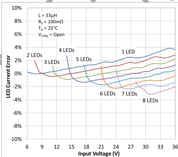
Figure 23. LED Current Deviation vs. Input Voltage
