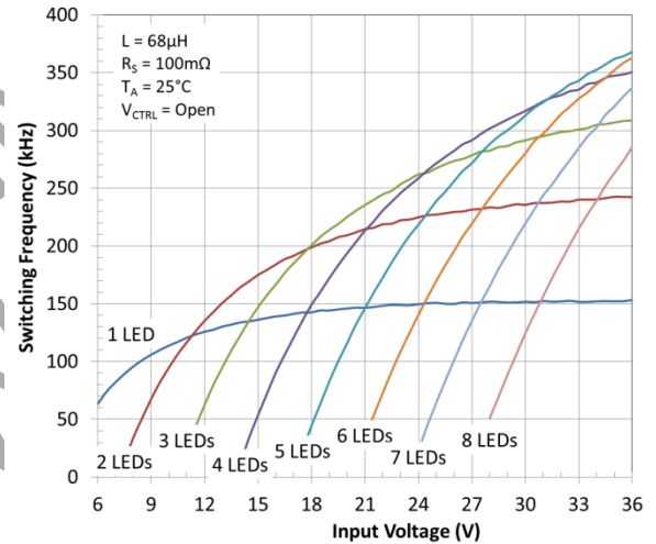
Figure 22. Switching Frequency vs. Input Voltage
