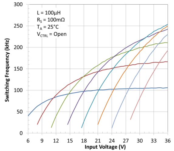
Figure 20. Switching Frequency vs. Input Voltage
