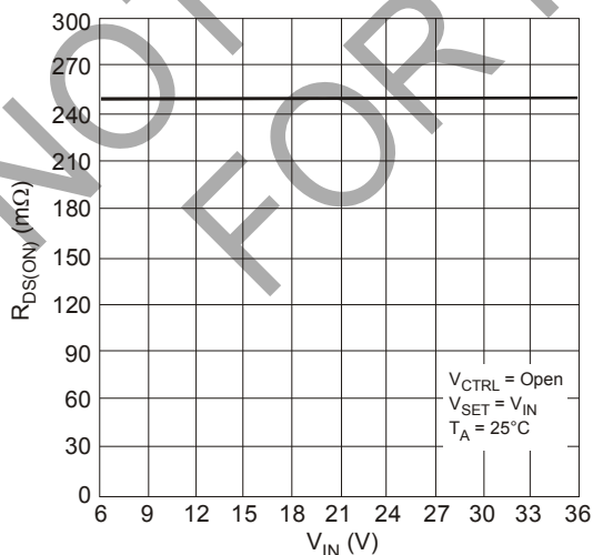
Figure 5 SW R_{DS(ON)} vs. Input Voltage
