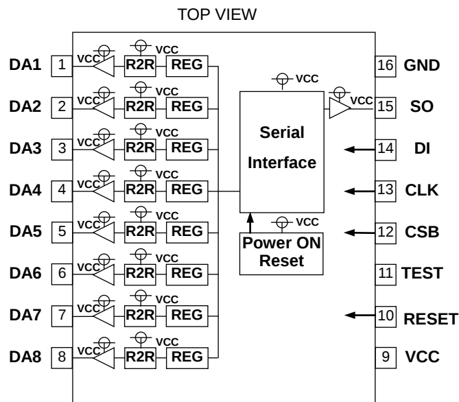
Figure 1. BH2226FV/BH2226F
