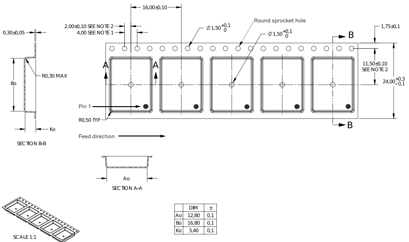
Figure 5: Dimensions (in mm) and orientation for NEO-M8 modules on tape
