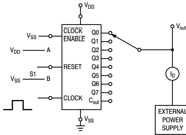
Figure 1. Typical Output Source and Output Sink Characteristics Test Circuit
